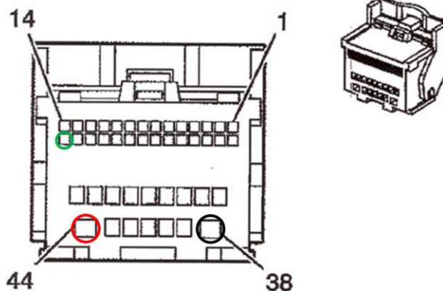
Pin definition female vehicle connector
