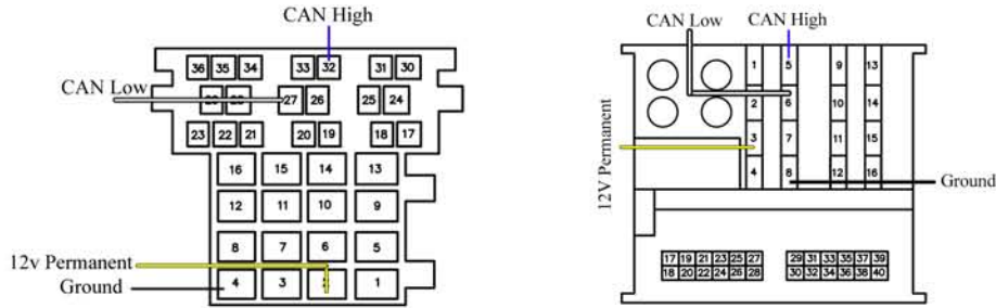
Quadlock (Fakra) CAN-Bus Vehicles
