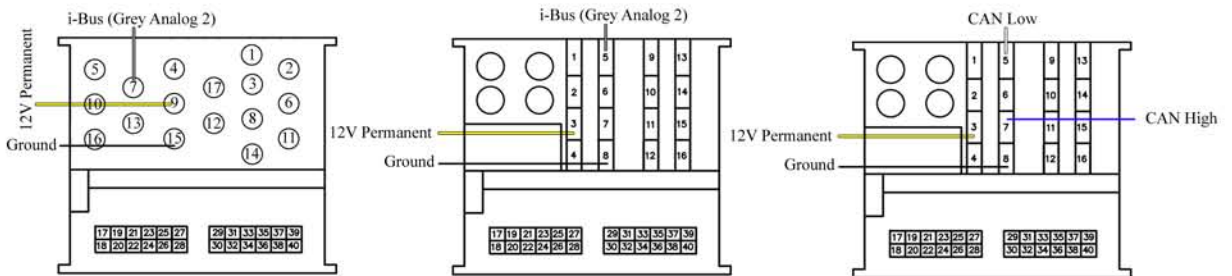
17 Way Round Pin i-Bus Vehicles
